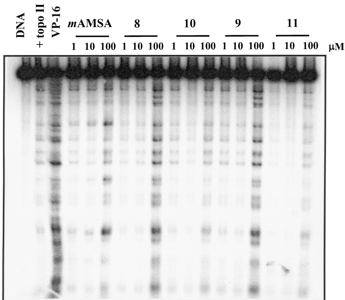
Figure 2. Topoisomerase II-stimulated DNA cleavage. The compounds tested were examined for their ability to stimulate human topoisomerase II-mediated DNA cleavage in the concentration range 1–100 \mu M. A representative gel showing the activity of the test compounds at three concentrations alongside with the reference compounds m -AMSA and etoposide (VP-16, 10 \mu M) is reported in the figure. The lane labelled DNA contains DNA alone, the lane labelled Topo II contains a mixture of DNA and topoisomerase II at the concentration used in the presence of drugs (1% DMSO in all tubes).
