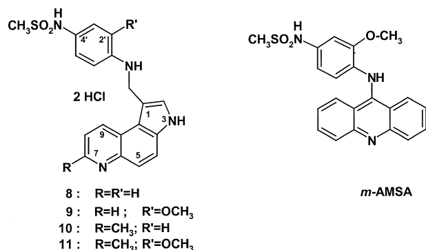
Figure 1. Chemical structure of the test pyrrolo-quinoline derivatives and m -AMSA.
